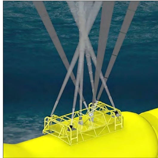
(b) Convergent Acoustic Doppler Profiler (C-ADP)
