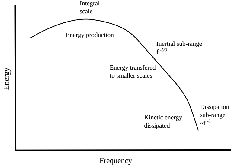
Figure 2.2: Illustration of the energy cascade highlighting the most important regions in tidal site characterisation. Adapted from [17].
