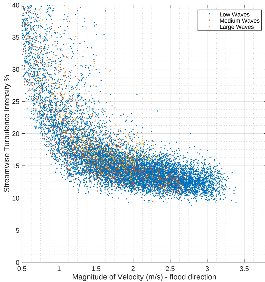
(a) Combination (inline ADCPs)
