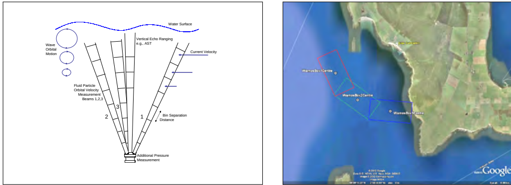
(a) Schematic showing principal of AWAC ADP in wave measurement mode. (b) Screenshot of map of Fall of Warne showing WaMoS regions of measurement. From EMEC (IPRTBC)).
